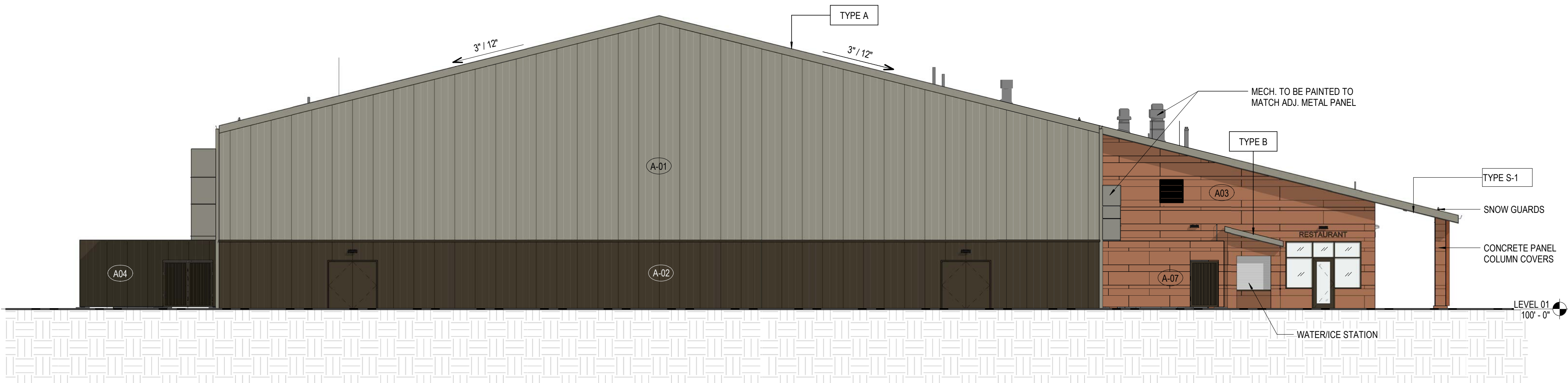
2 BUILDING ELEVATION - EAST 3/32" = 1'-0"
