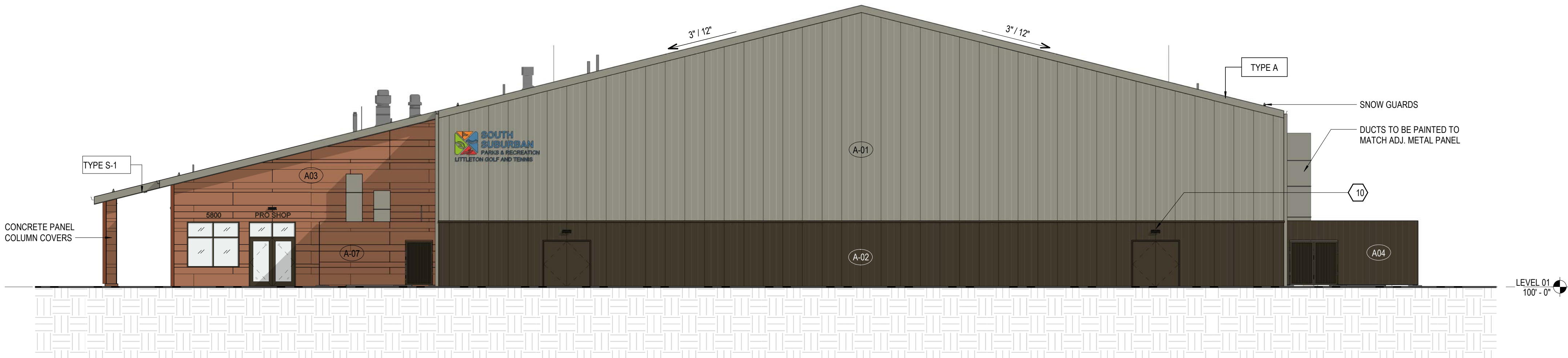
2 BUILDING ELEVATION - WEST 3/32" = 1'-0"
